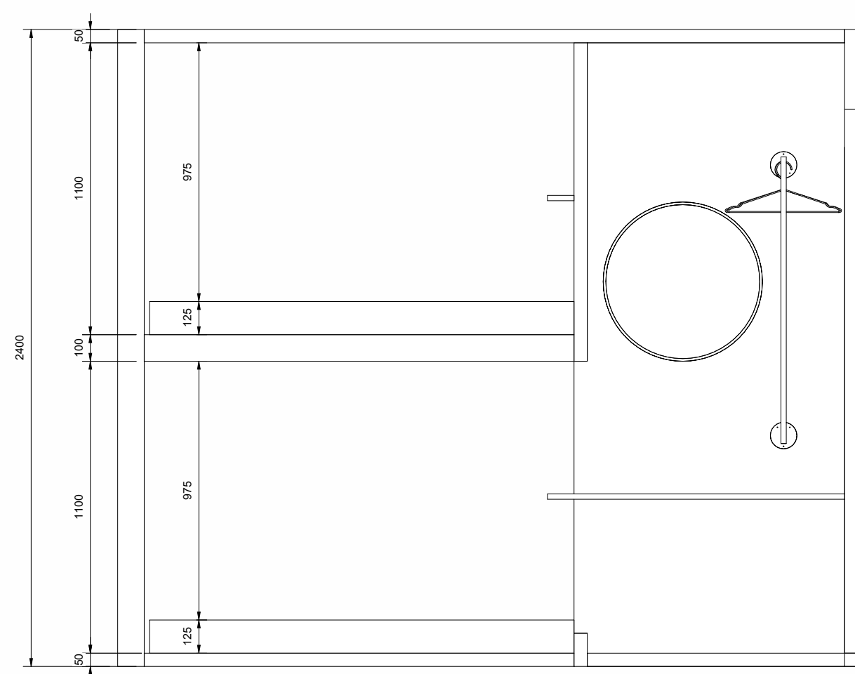
3 Interior side 1 : 20
