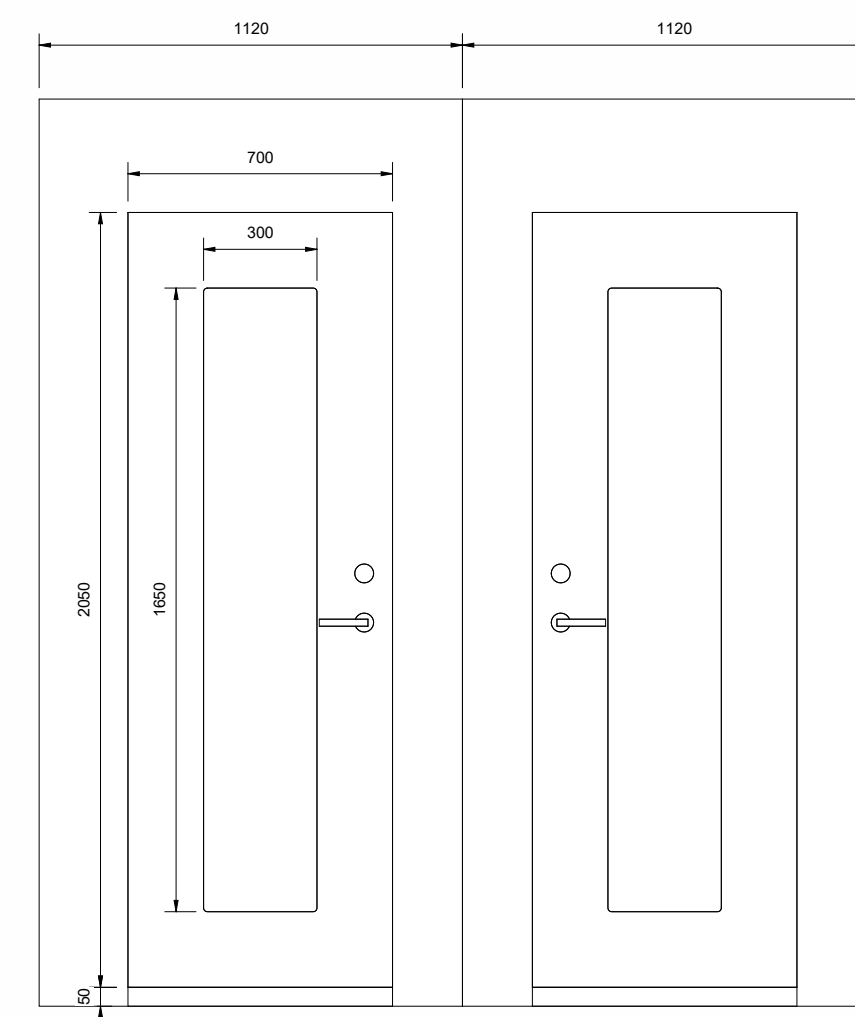
4 Exterior front 1 : 20
